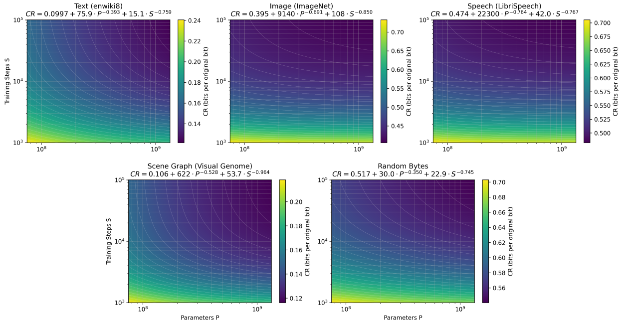
Figure 1: Scaling laws for LLM compression across text, image, speech, scene graph, and random byte modalities. The heatmaps show compression ratio as a function of model parameters ( P ) and training steps ( S ). Lower compression ratios (darker colors) indicate better compression performance. Each modality follows the power law CR(P, S) = a + bP^{-\alpha} + cS^{-\beta} with modality-specific coefficients shown in the equations above each subplot.
